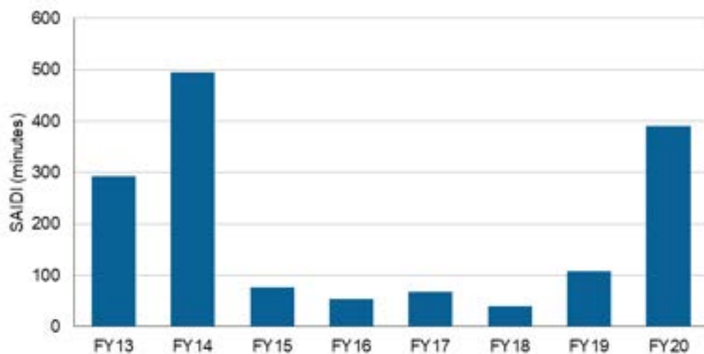
Figure 6.5: Average minutes off supply (SAIDI) for the Pilbara network, 2013 to 2020
