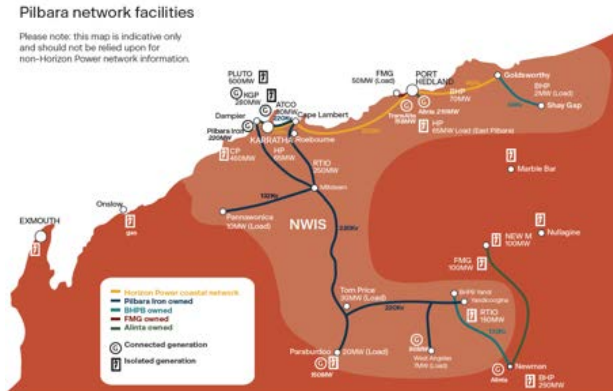
Figure 1: Horizon Power coastal network and surrounding networks
